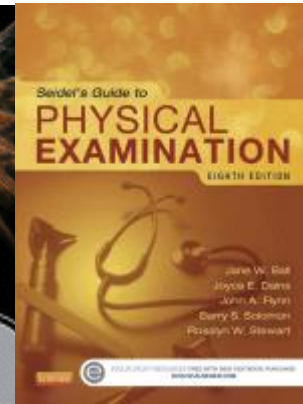
Seidel's
